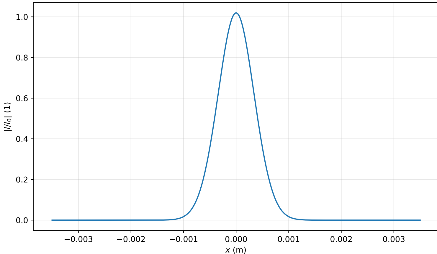
Intensity profile I(x, y = 0, z = 0.159m)/I_0 , P_{in}=1.0P_{cr} , artificial time
